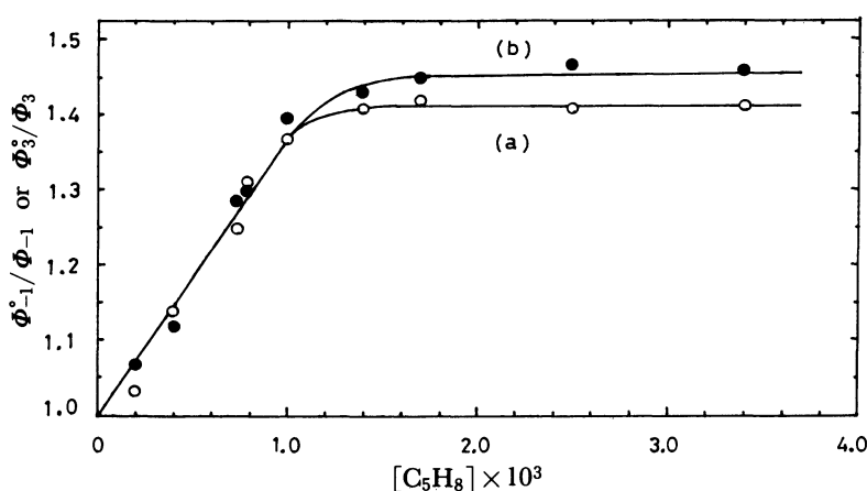
Fig. 2. Triplet quenching of the photosubstitution reaction (1→3) in cyclohexane. [1]=1.62 \times 10^{-3} \text{ mol dm}^{-3} . (a) —○—: \phi_3^0/\phi_3 , (b) —●—: \phi_3^0/\phi_1 .
